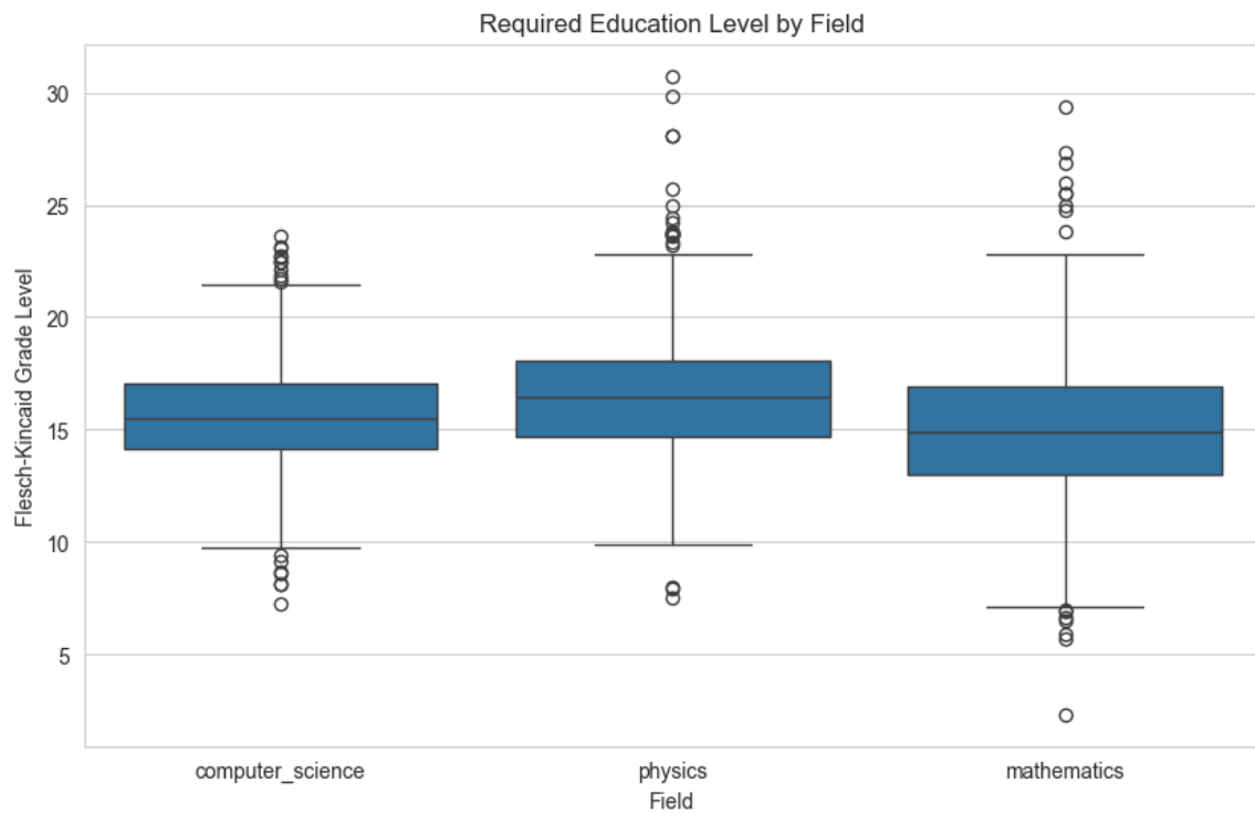
Figure 3. Flesch-Kincaid Grade Level across Fields—Box Plots
