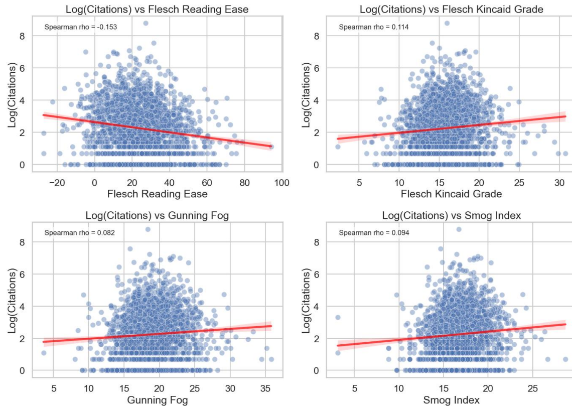
Figure 4. Scatter plots of \log(\text{Citations} + 1) against each of the four readability metrics
