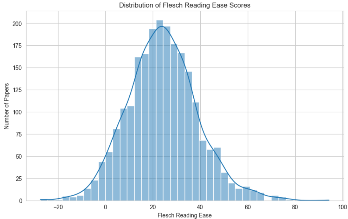
Figure 1. Distribution of Flesch Reading Ease scores across the full dataset
