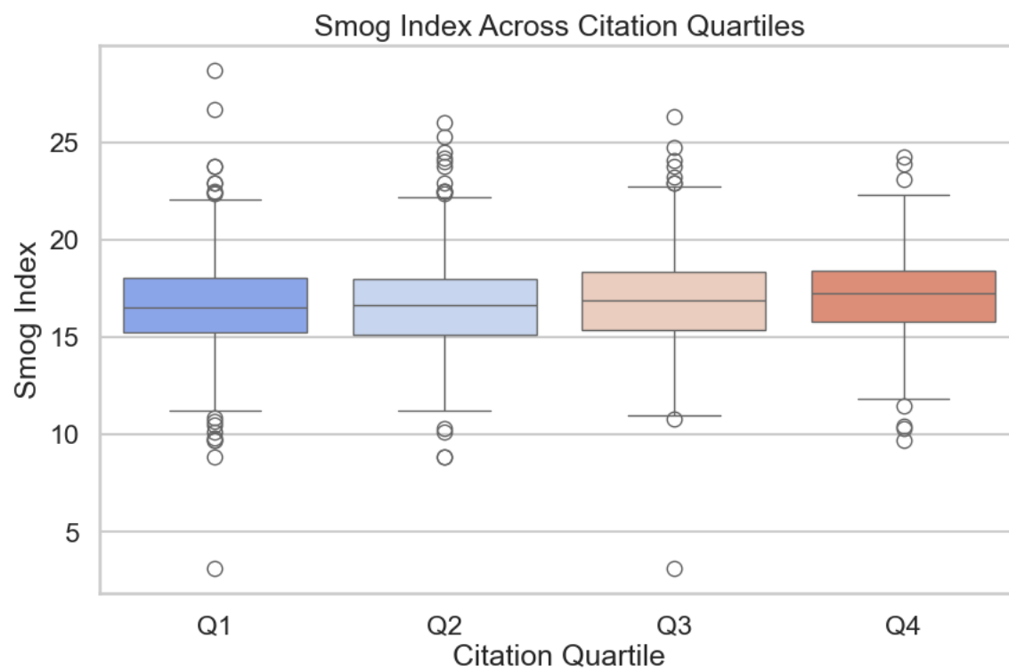
Figure 8. Smog index scores across citation quartiles (Q1 = lowest 25% of citation counts; Q4 = highest 25%).
