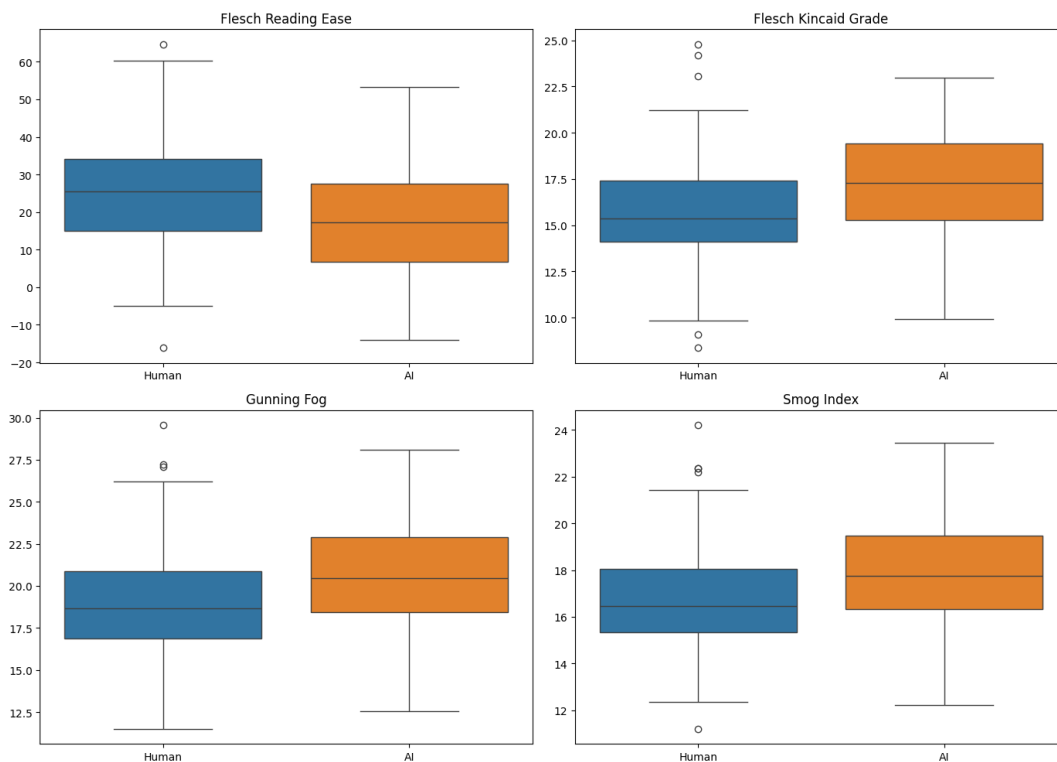
Figure 11. Side-by-side boxplots comparing the full distributions of human-authored (blue) and AI-generated (orange) abstracts across all four readability metrics (n = 150 pairs).
