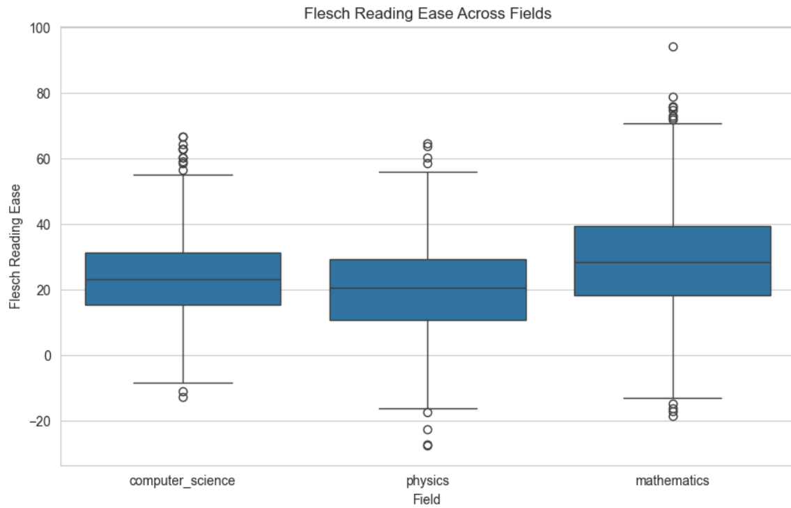
Figure 2. Flesch Reading Ease across Fields—Box Plots
