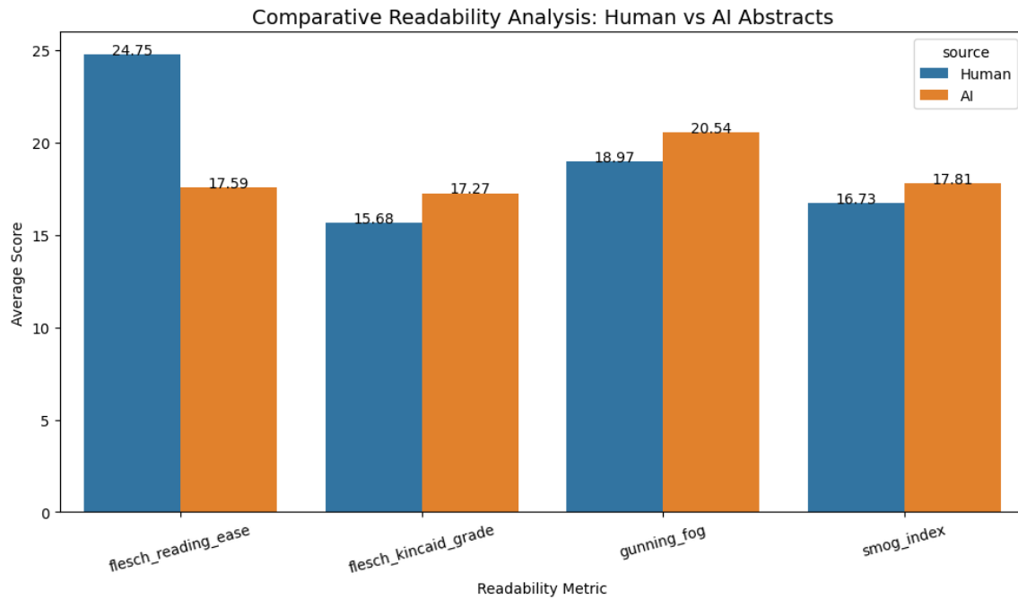
Figure 9. Comparative bar chart of mean readability scores for human-authored and AI-generated abstracts ( n = 150 pairs)
