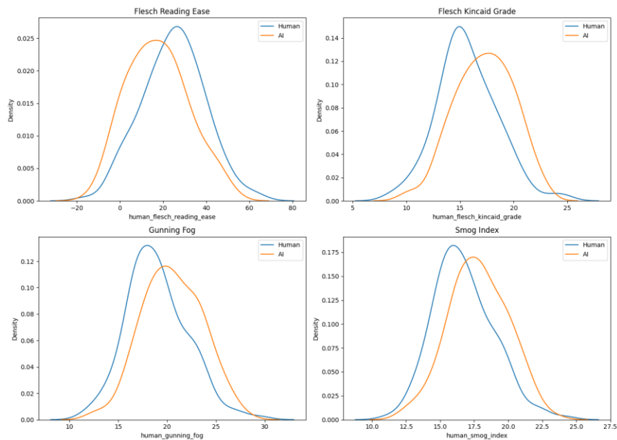
Figure 10. Distributional Comparison of Readability Metrics: Human vs. AI-Generated Scientific Abstracts
